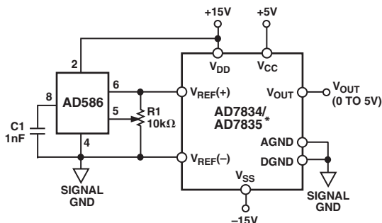
Figure 4. Unipolar 5 V Operation
