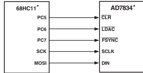
Figure 12. AD7834 to 68HC11 Interface
