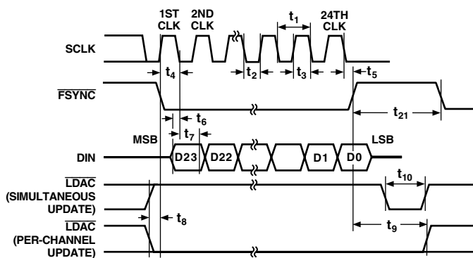
Figure 1. AD7834 Timing Diagram
