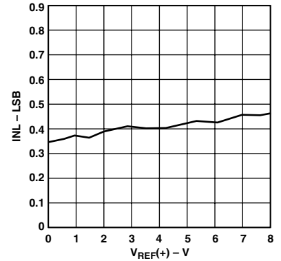
TPC 3. Typical INL vs. V_{REF}(+) ( V_{REF}(-) = -6\text{ V} )
