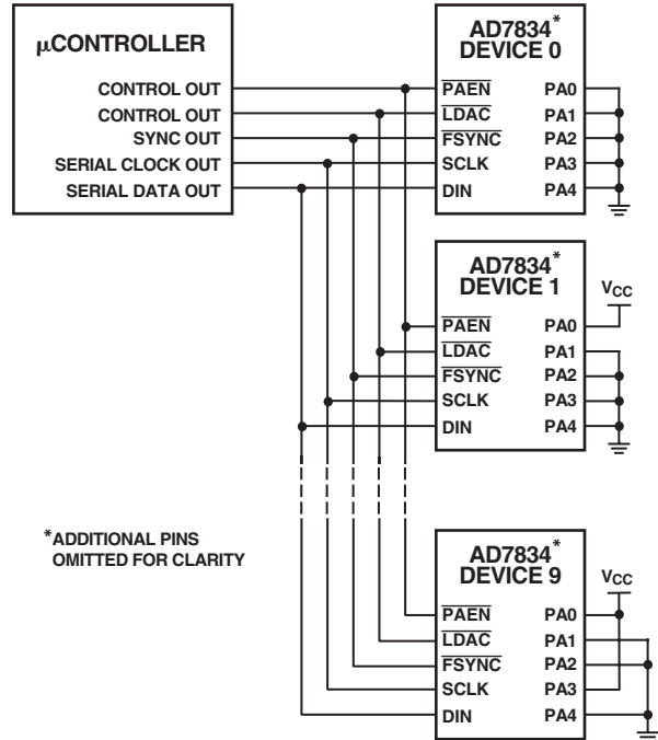
Figure 18. Serial Interface to Multiple AD7834s
