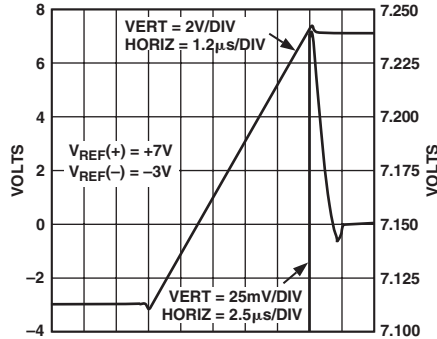
TPC 8. Settling Time (+)
