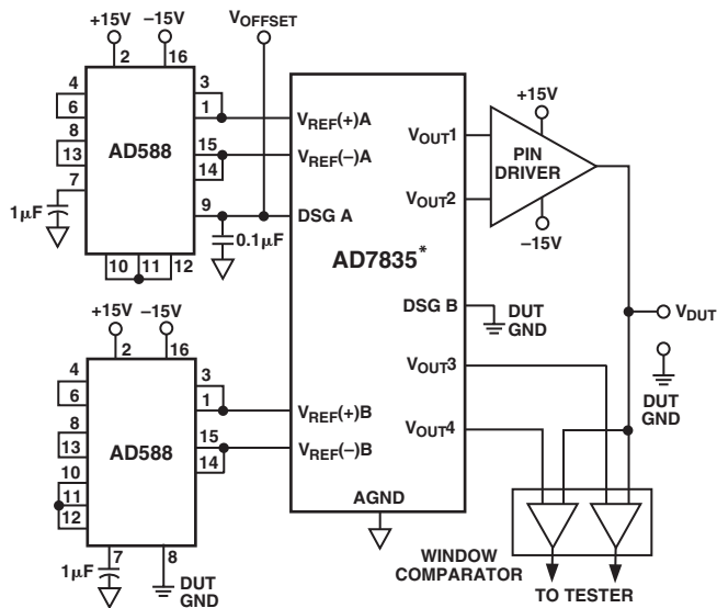
Figure 20. ATE Application
