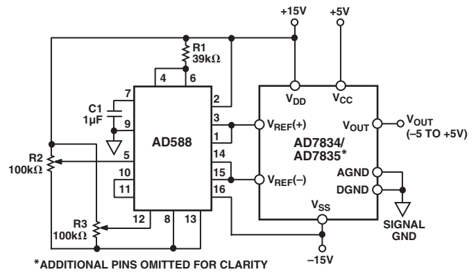
Figure 5. Bipolar \pm 5 V Operation
