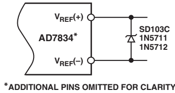
Figure 10. Power-On Protection
