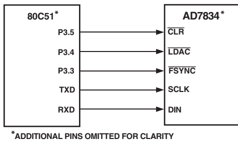
Figure 11. AD7834 to 80C51 Interface
