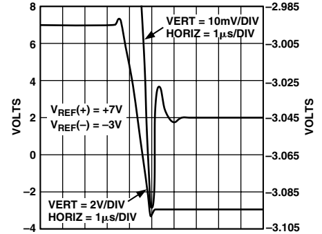
TPC 9. Settling Time (-)
