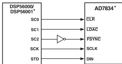
Figure 14. AD7834 to DSP56000/DSP56001 Interface
