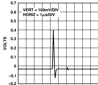
TPC 7. Typical Digital/Analog Glitch Impulse
