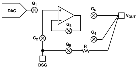
Figure 7. Output Stage with V_{DD} < 10 V
