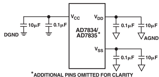
Figure 21. Power Supply Decoupling
