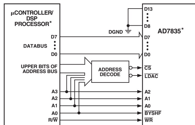
Figure 17. AD7835 8-Bit Interface
