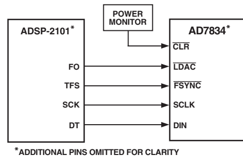
Figure 13. AD7834 to ADSP-2101 Interface
