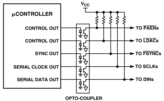
Figure 19. Opto-Isolated Interface
