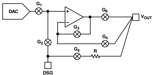
Figure 6. Block Diagram of AD7834/AD7835 Output Stage
