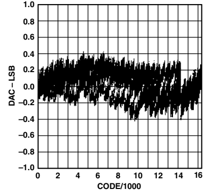
TPC 6. Typical DAC-to-DAC Matching
