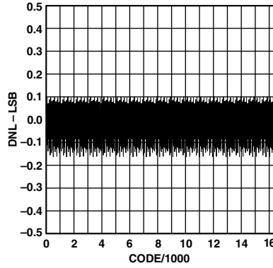
TPC 2. Typical DNL Plot
