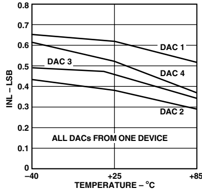
TPC 5. Typical INL vs. Temperature
