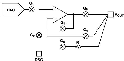
Figure 8. Output Stage with V_{DD} > 10 V and \overline{CLR} Low
