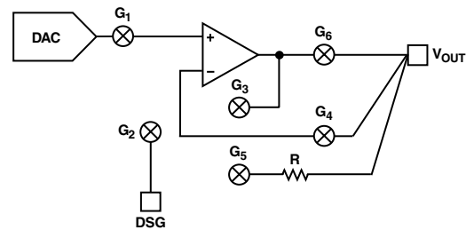
Figure 9. Output Stage with \overline{LDAC} Low
