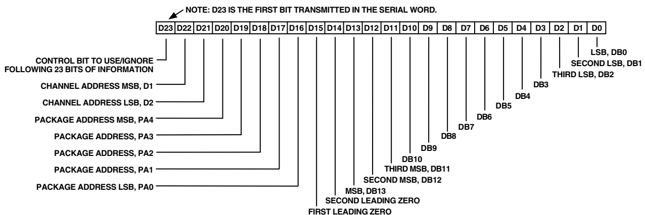
Figure 3. Bit Assignments for 24-Bit Data Stream of AD7834
