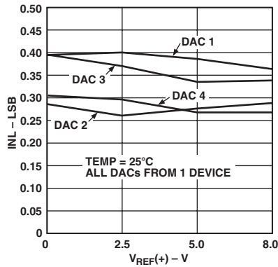
TPC 4. Typical INL vs. V_{REF}(+) ( V_{REF}(+) - V_{REF}(-) = 5\text{ V} )
