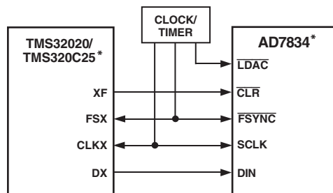
Figure 15. AD7834 to TMS32020/TMS320C25 Interface
